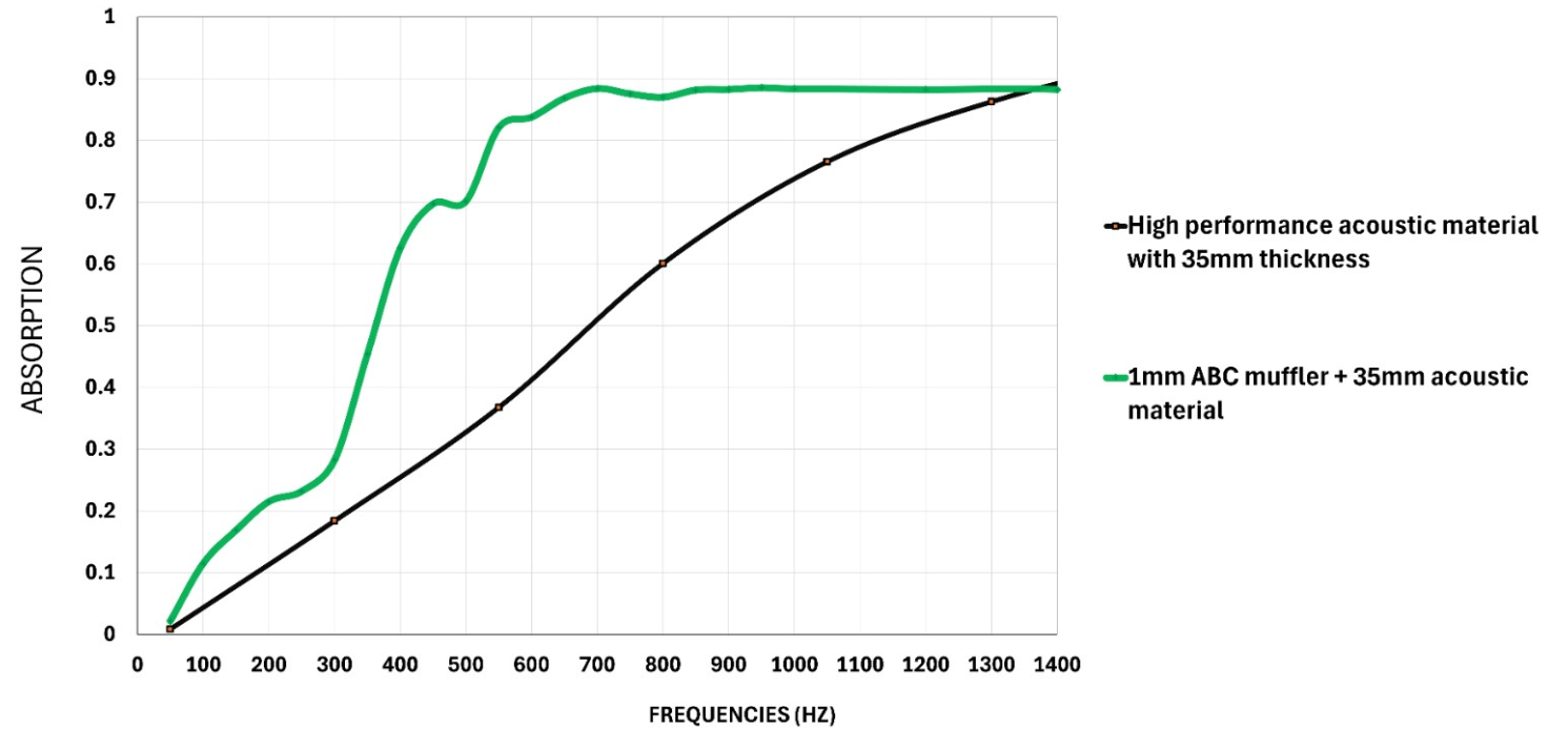
RESULT OF IMPROVED ACOUSTIC MATERIAL ABSORPTION
